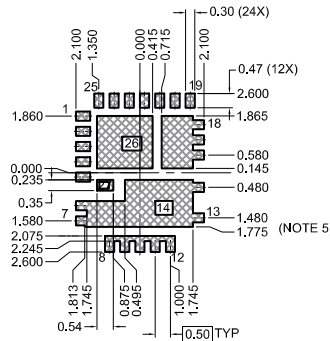
RECOMMENDED MOUNTING FOOTPRINT
