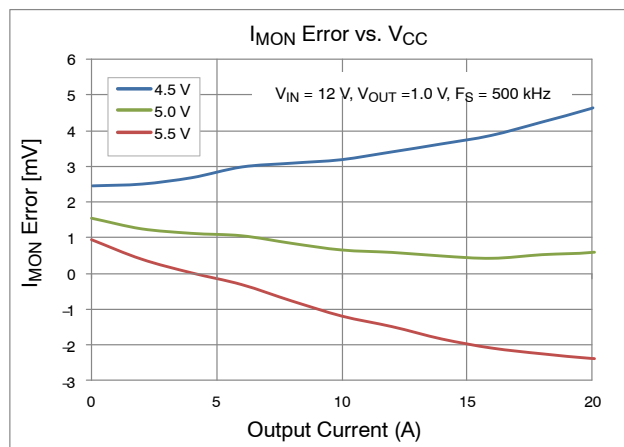
Figure 23. IMON Accuracy vs. V_{CC}
