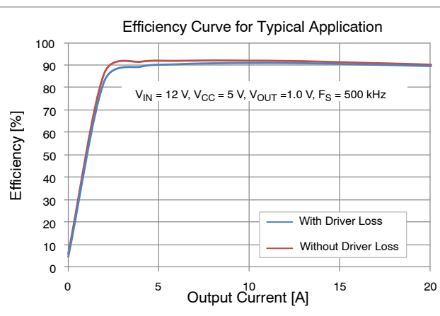
Figure 24. Efficiency Curve for Typical Application
