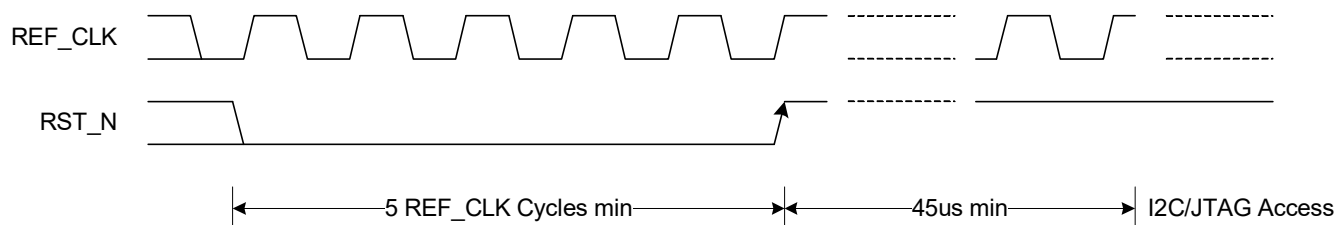
Figure 23: Reset Timing
