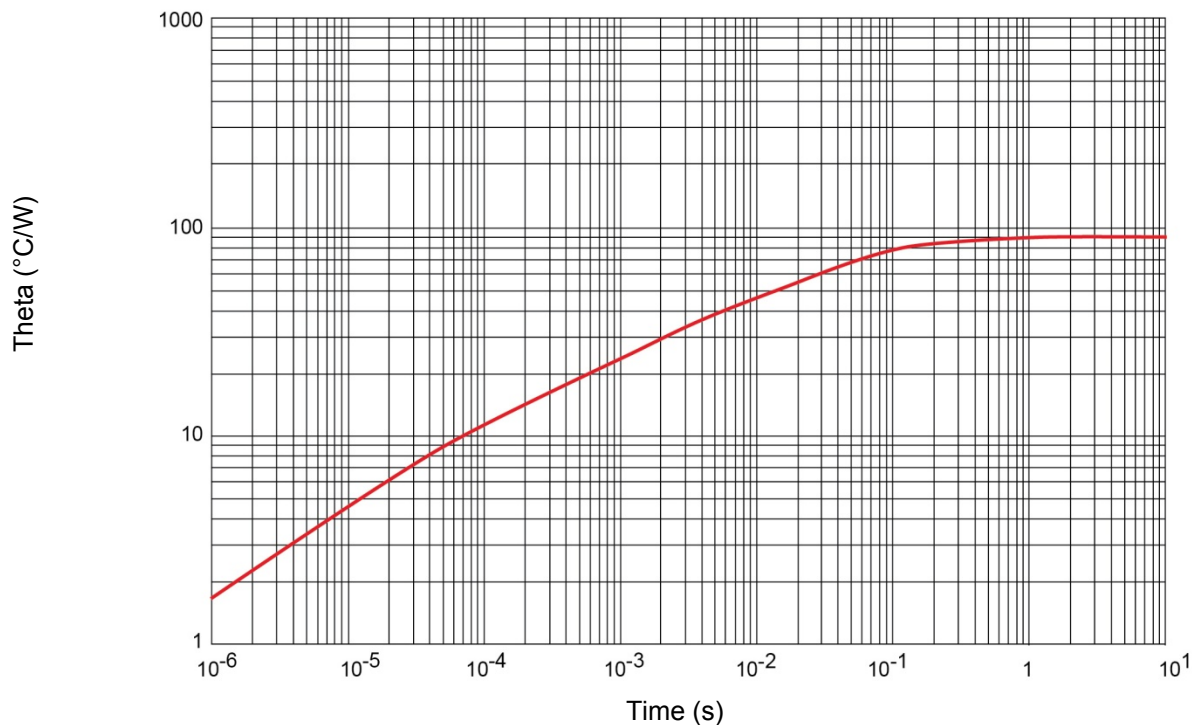
FIGURE 2 Thermal impedance graph ( R_{\theta JSP(IS)} )
