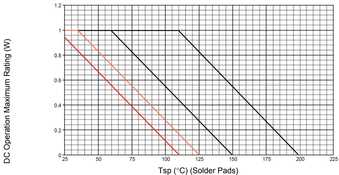
FIGURE 1 Temperature-Power Derating (Infinite sink mount to PCB)
