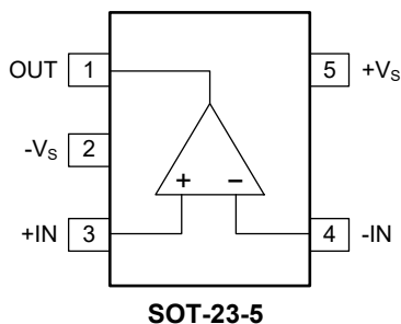
SGM8958-1 (TOP VIEW)
