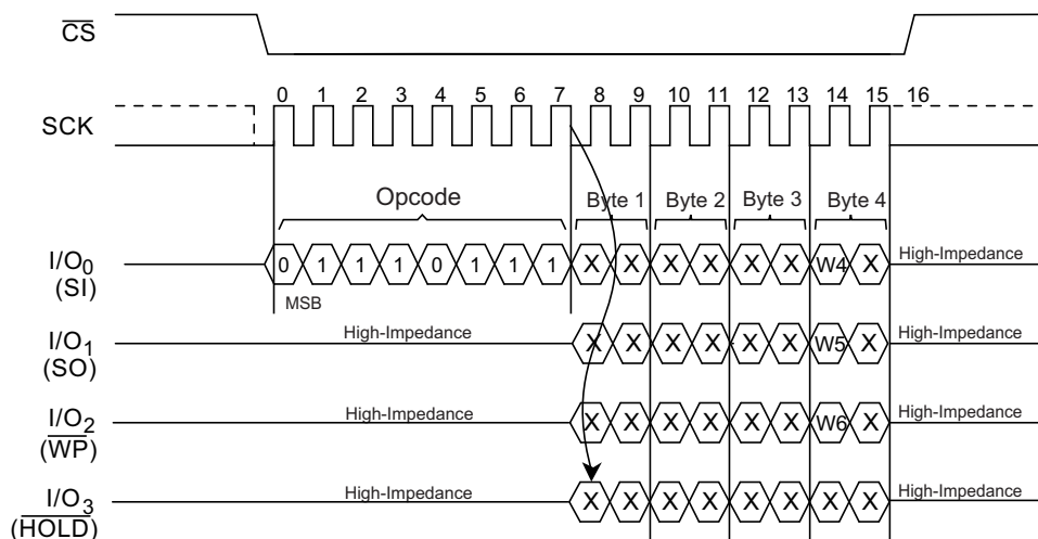
The Set Burst with Wrap command sequence is: \overline{\text{CS}} goes low \rightarrow Send Set Burst with Wrap command \rightarrow Send 24 Dummy bits \rightarrow Send 8 "Wrap bits" \rightarrow \overline{\text{CS}} goes high.
