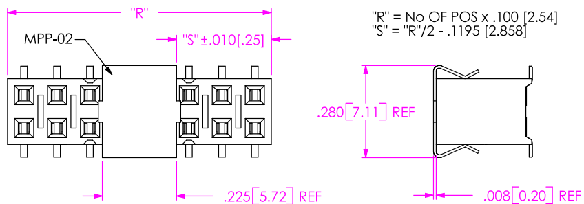
FIGURE 5 -M: METAL PICK & PLACE PAD
