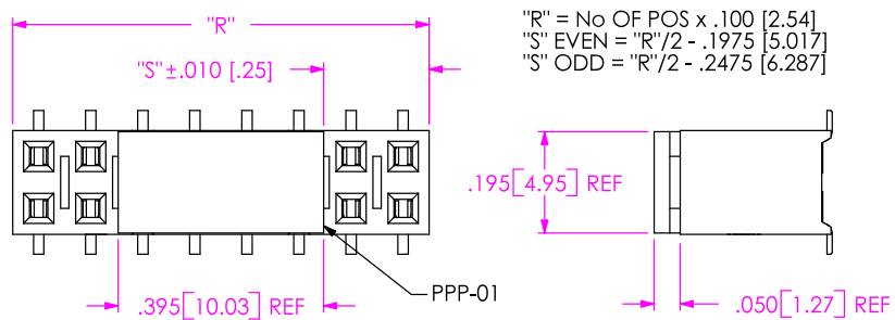
FIGURE 4 -P: PICK & PLACE PAD
