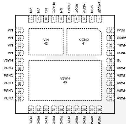
Figure 4. Top View
