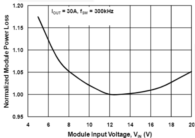
Figure 10. Normalized Power Loss vs. Input Voltage
