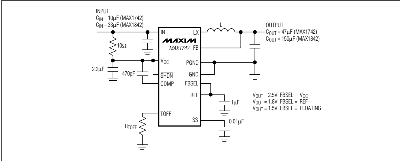
Figure 1. Typical Circuit
