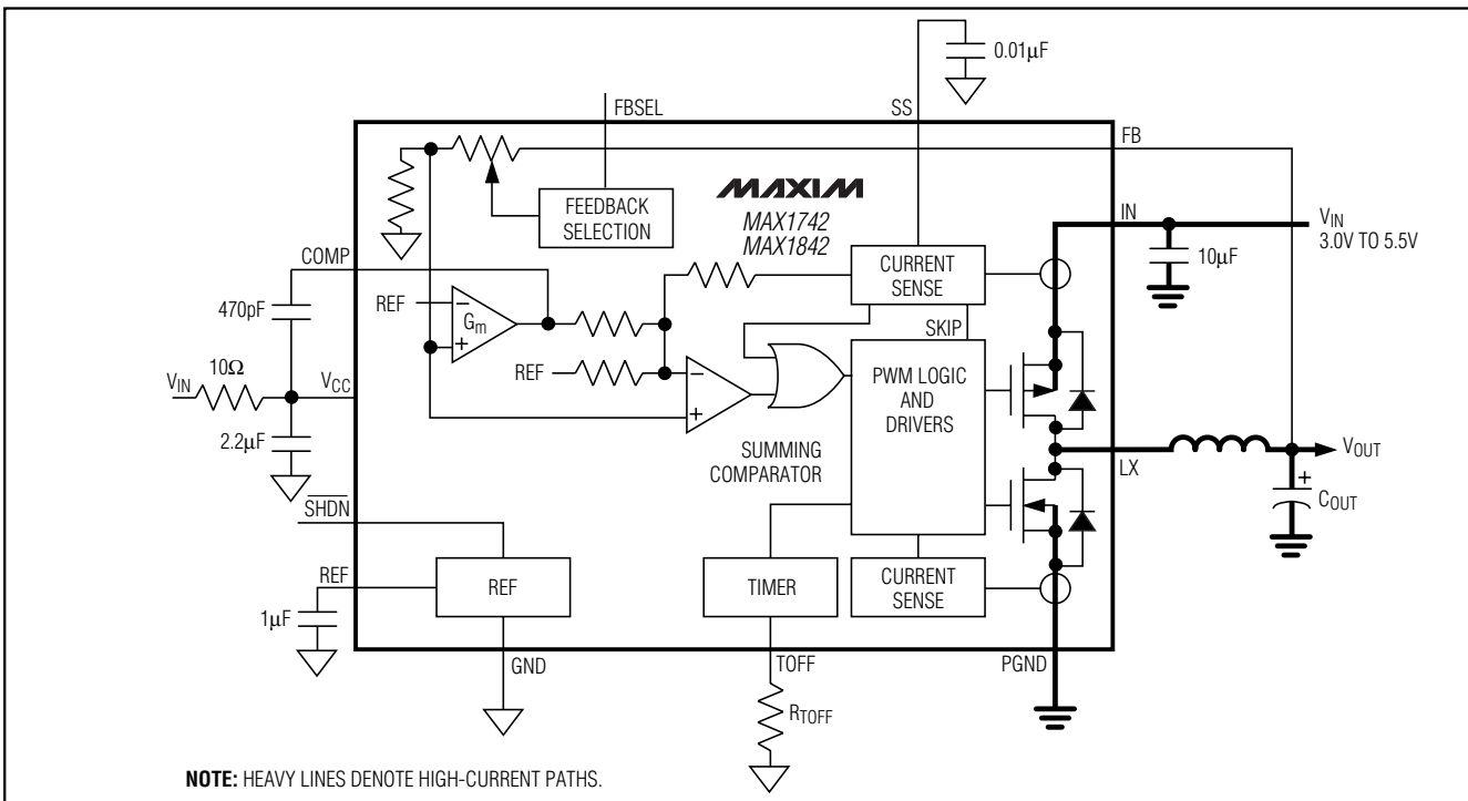
Figure 2. Functional Diagram
