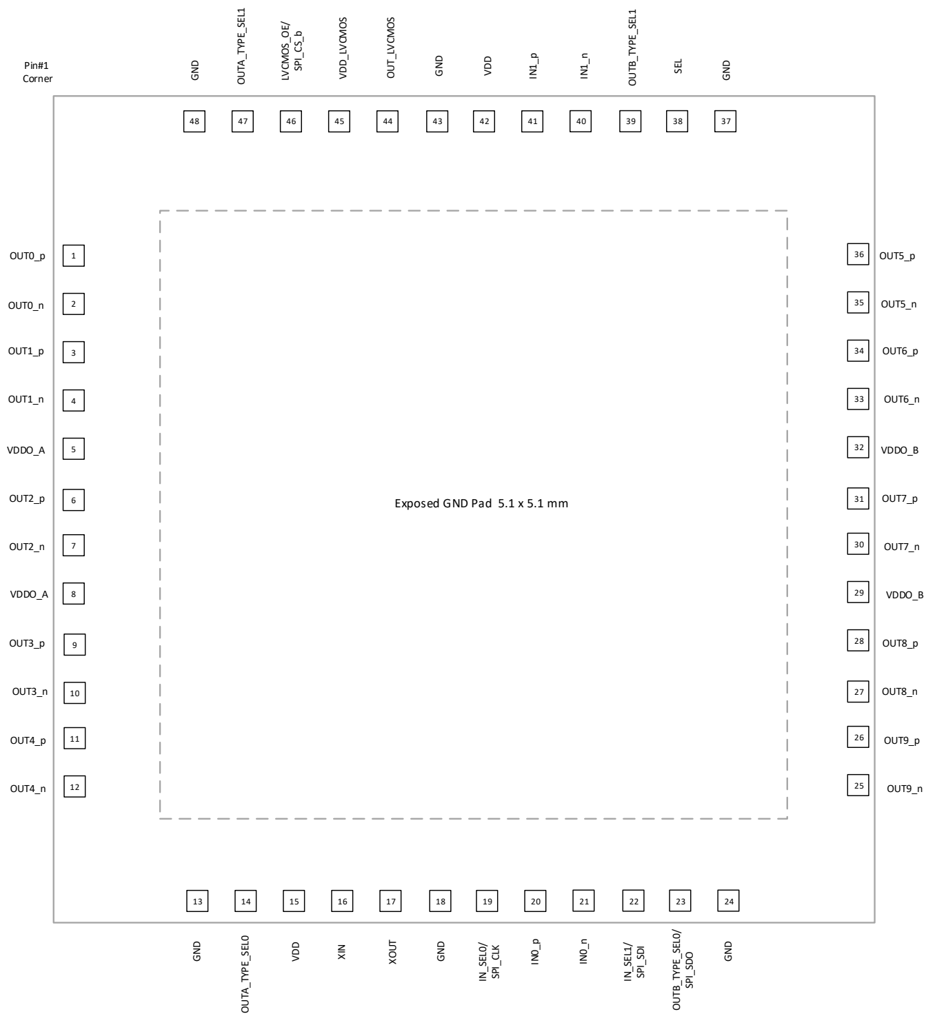
Figure 2. Pin Diagram
