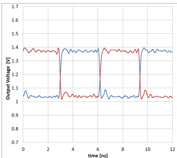
Figure 21. 156.25MHz LVDS
