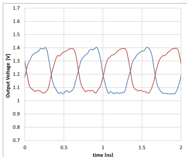
Figure 22. 1.5GHz LVDS
