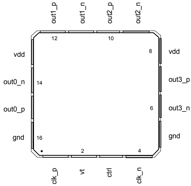
Figure 2 - Pin Connections
