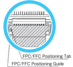
Correct Insertion
