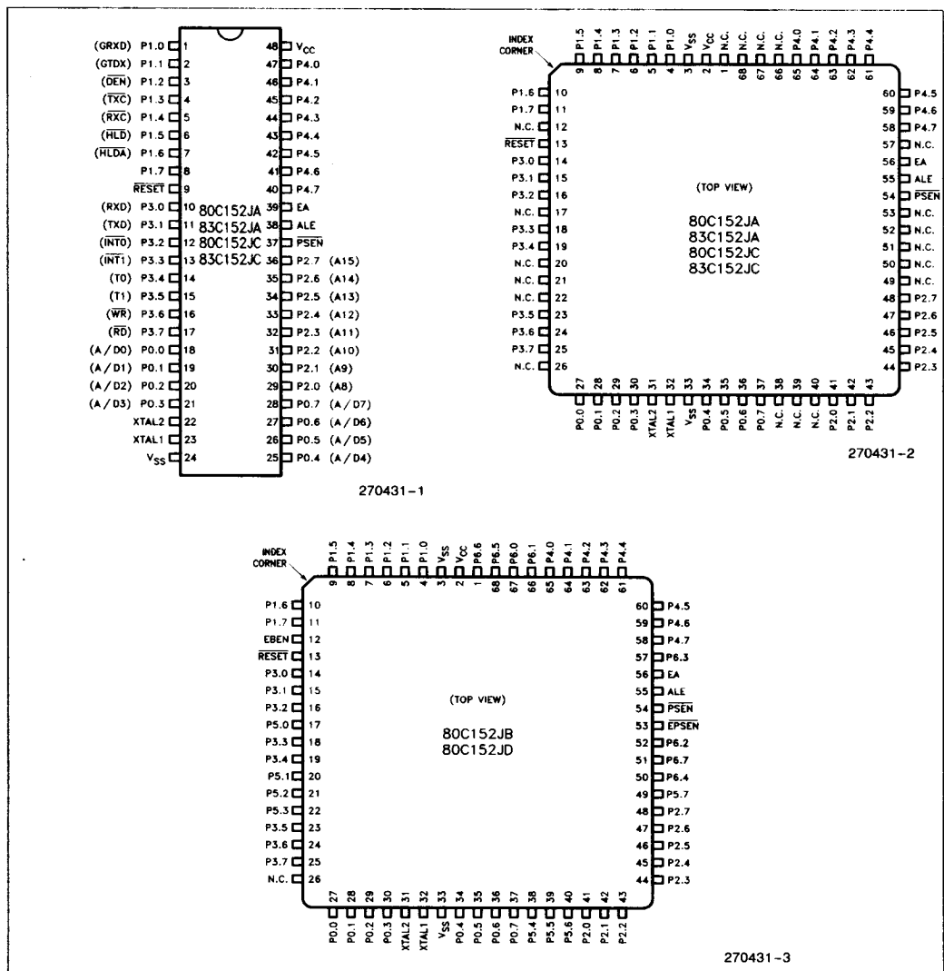
Figure 1. Connection Diagrams
