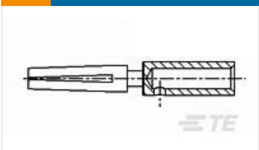
TE Part #5-1437720-7 T01-CRIMP-S05=TRIAD
