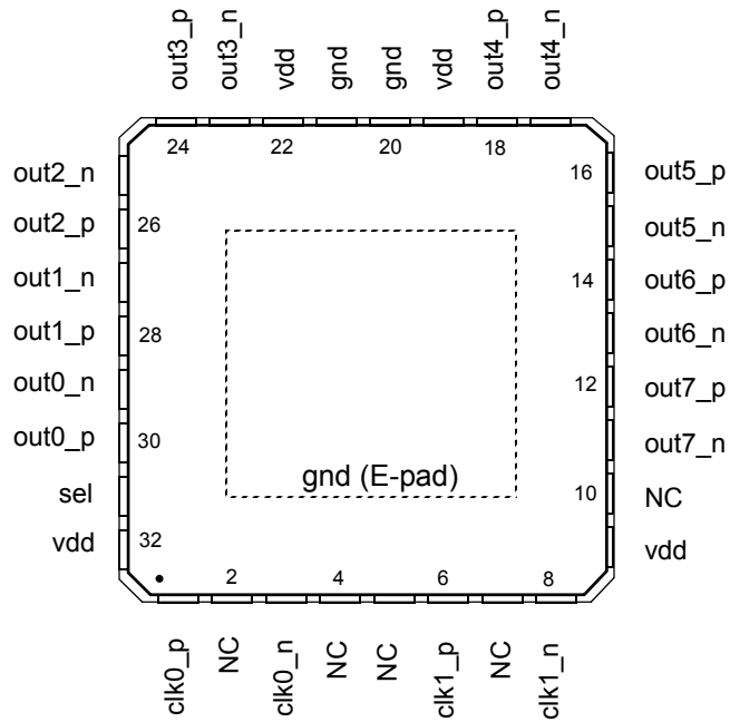
Figure 2 - Pin Connections
