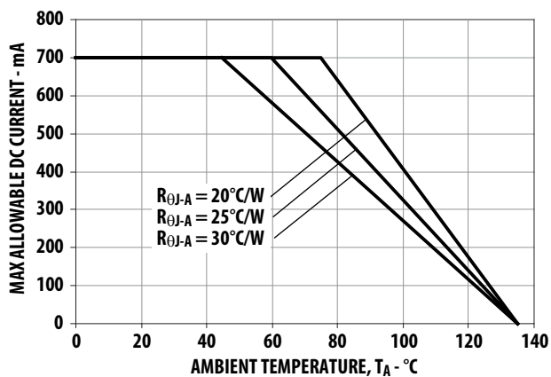
Figure 13 Maximum Forward Current vs. Ambient Temperature. Derated based on T_{J\text{MAX}} = 125^{\circ}\text{C} , R_{\theta J-A} = 20^{\circ}\text{C/W} , 25^{\circ}\text{C/W} , and 30^{\circ}\text{C/W} .
