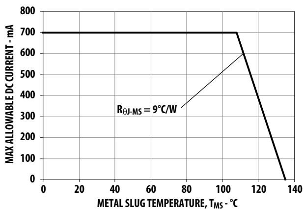
Figure 14 Maximum Forward Current vs. Metal Slug Temperature. Derated based on T_{J\text{MAX}} = 125^{\circ}\text{C} , R_{\theta J-MS} = 9^{\circ}\text{C/W} .
