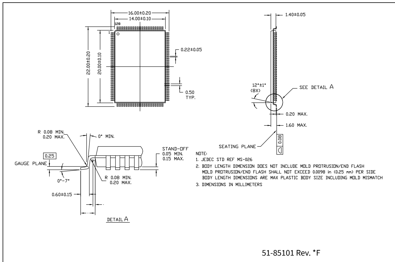
Figure 18 A128RA package outline (PG-TQFP-128), 51-85101
