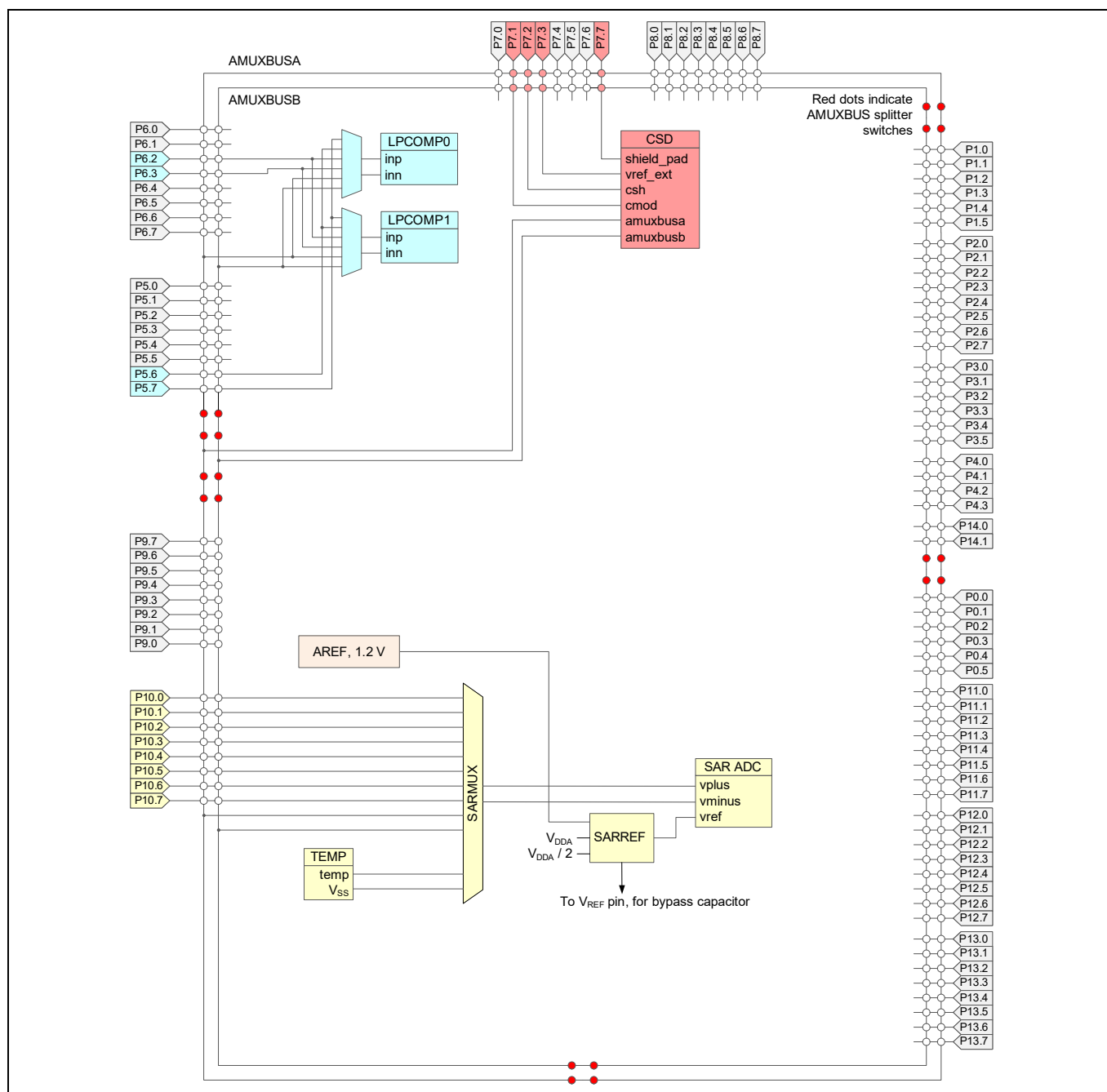
Figure 6 Analog subsystem
