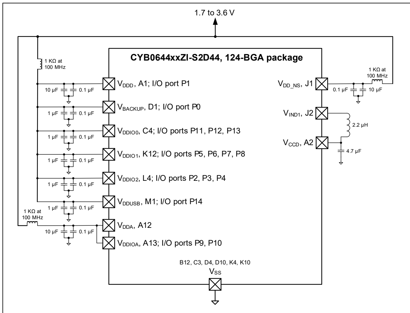
Figure 13 124-BGA Power Connection Diagram
