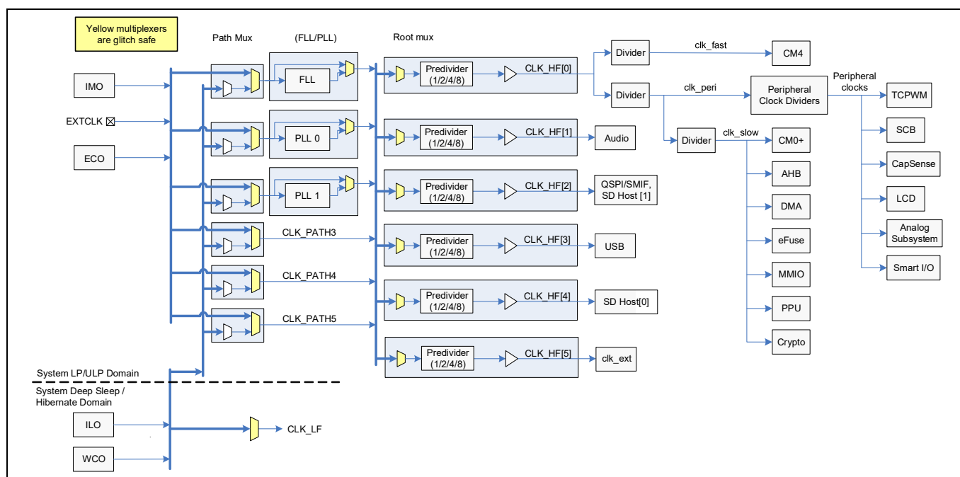
Figure 3 Clocking diagram
