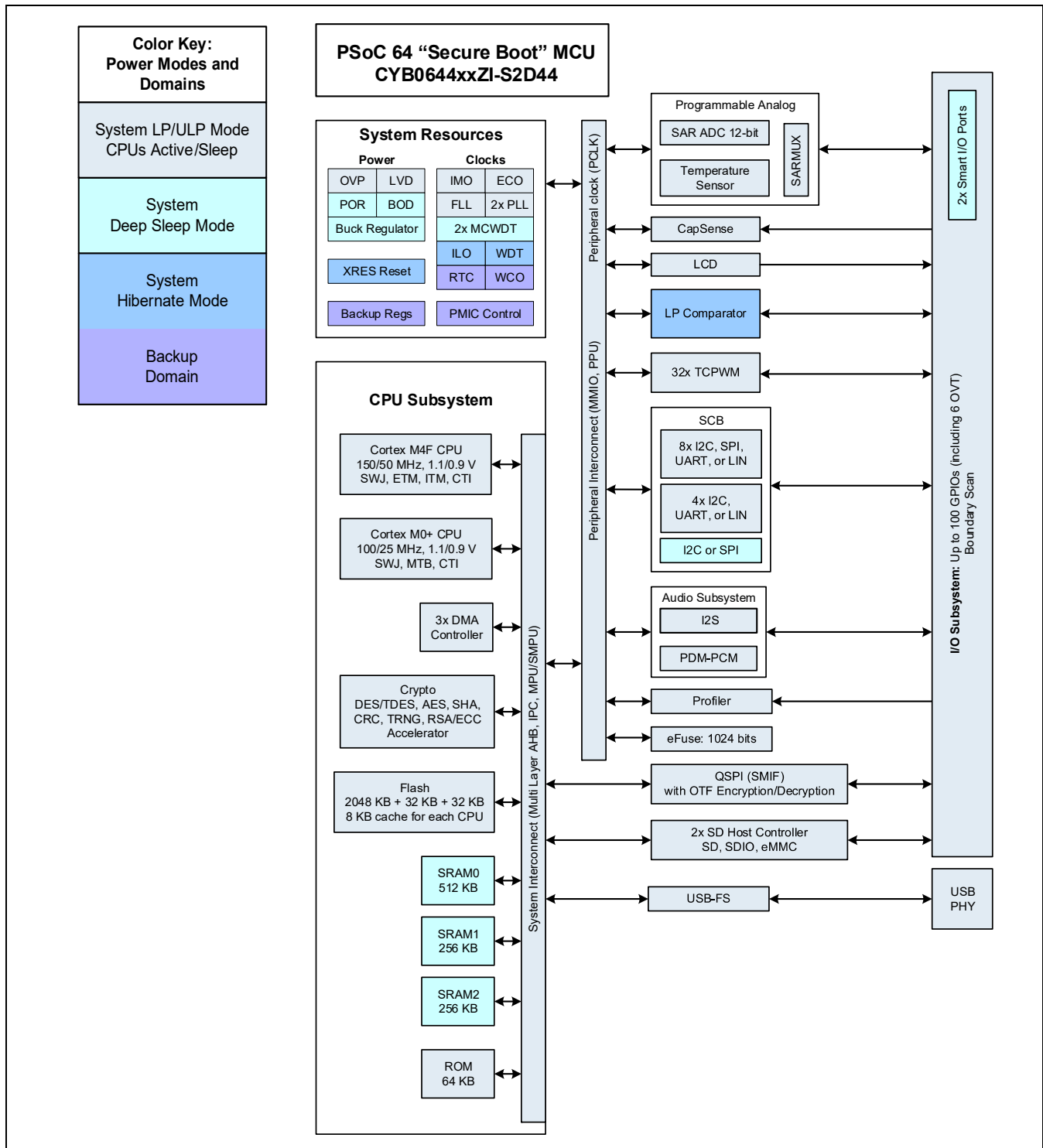
Figure 2 Block Diagram
