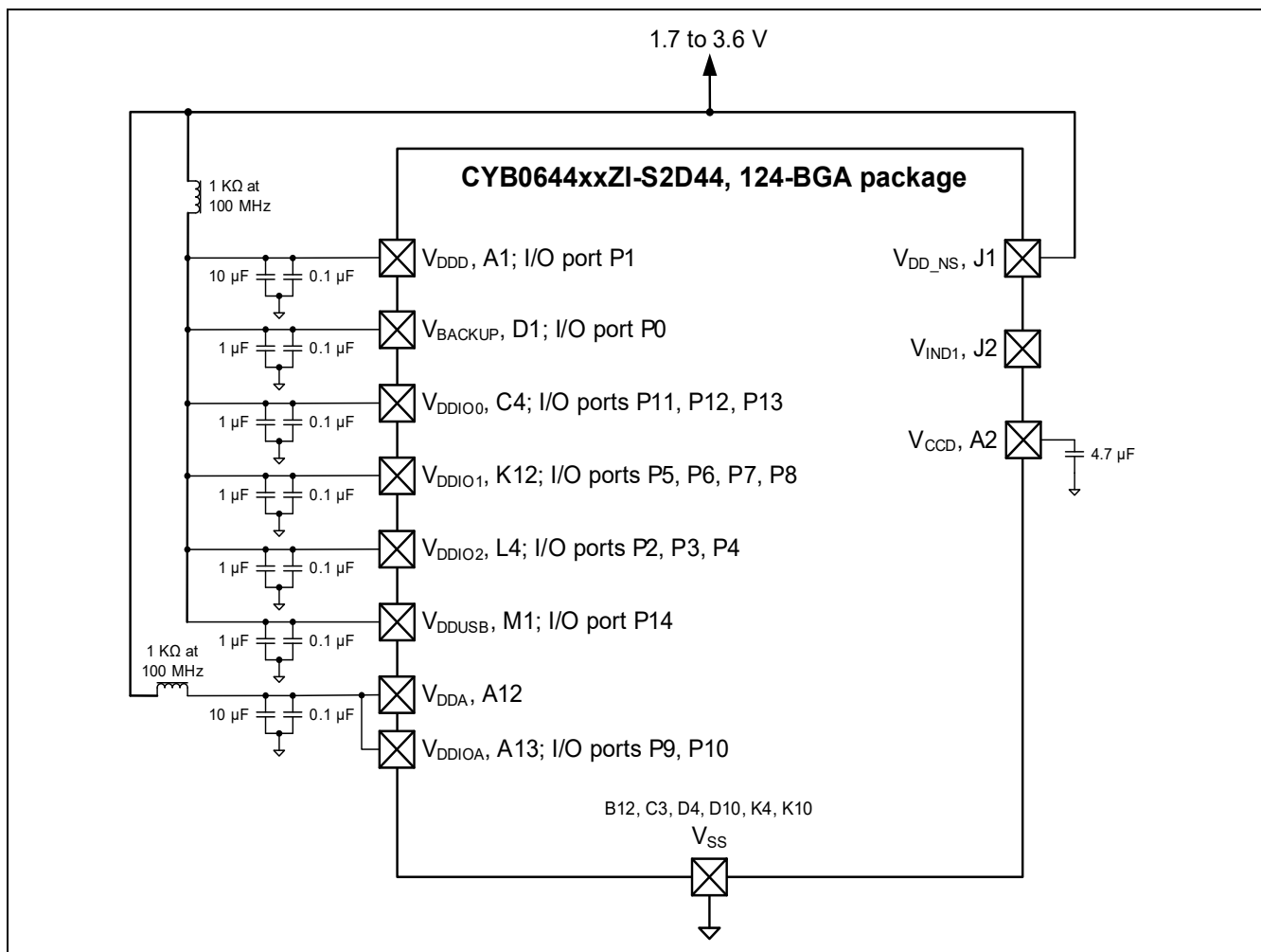
Figure 14 124-BGA (No Buck) Power Connection Diagram
