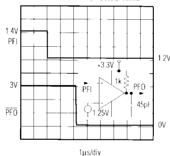
POWER-FAIL COMPARATOR ASSERTION RESPONSE TIME
