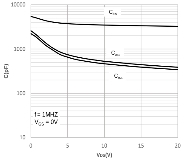
Figure 6: Capacitance Characteristics
