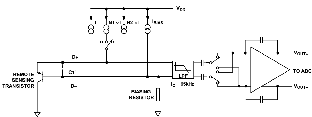
Figure 12. Input Signal Conditioning
