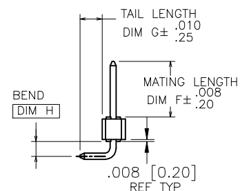
END VIEW
