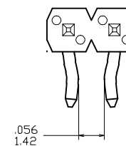
DETAIL N NOTE 8
