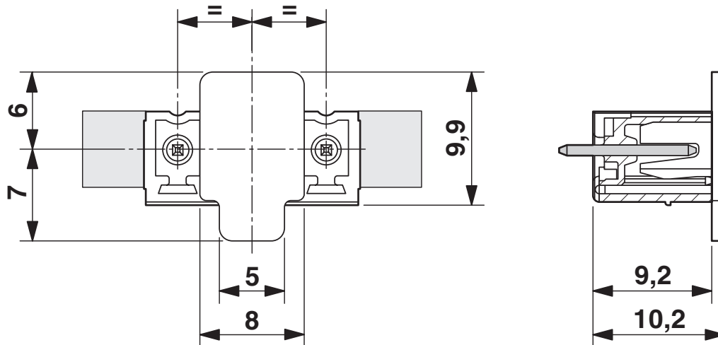
Drilling plan/solder pad geometry
