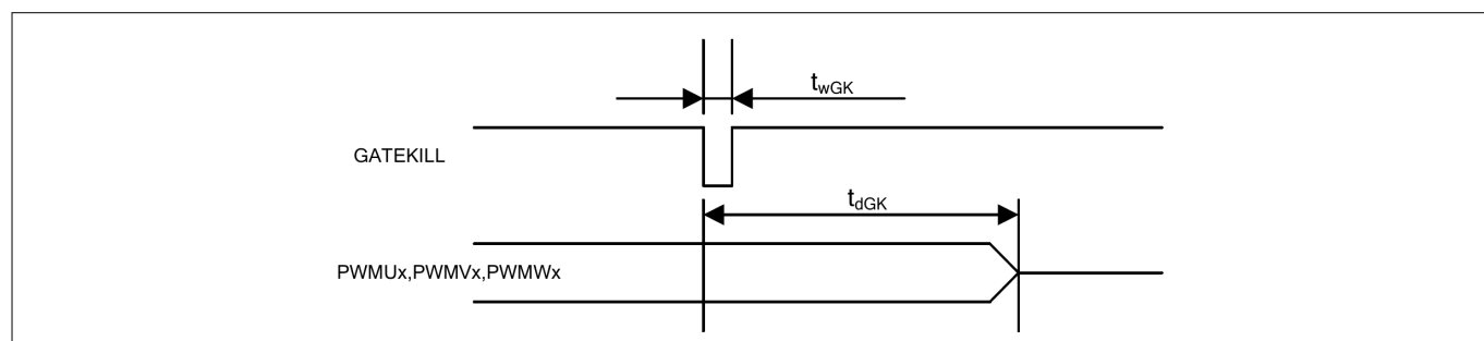
Figure 15 Fault timing
