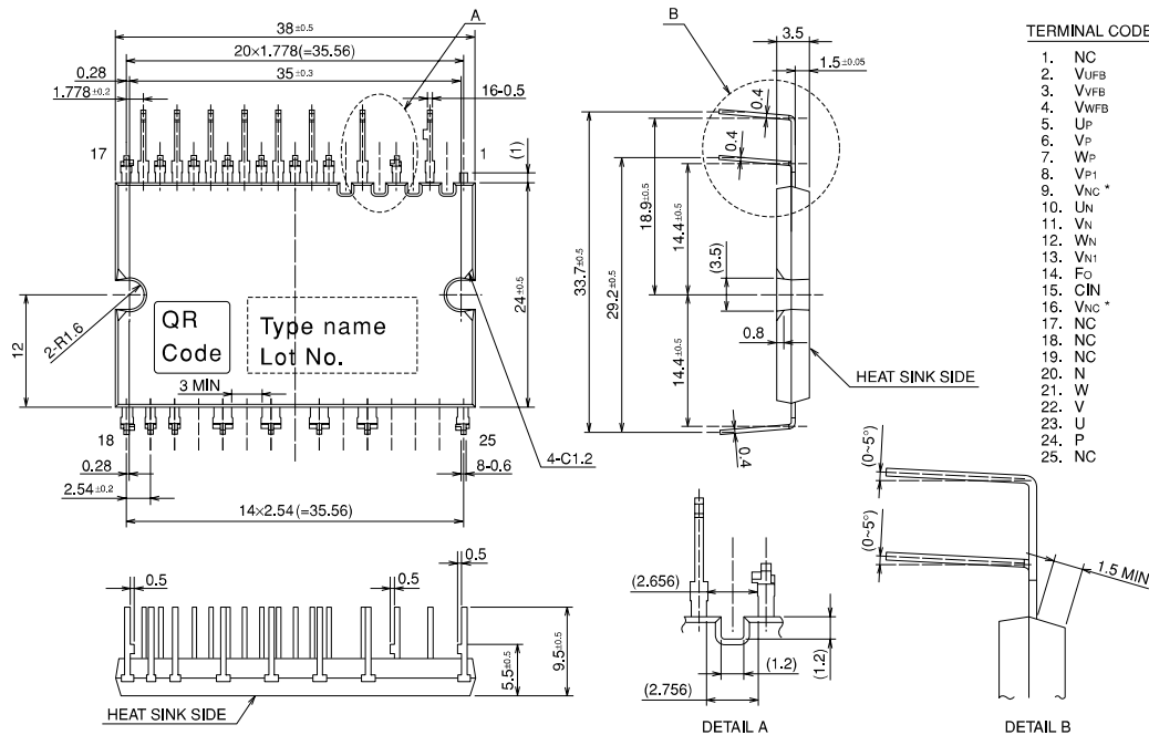
Fig. 3 ZIGZAG TERMINAL TYPE PACKAGE OUTLINES (PS21965-4C)
