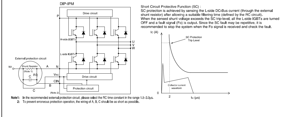
Fig. 6 EXTERNAL PART OF THE DIP-IPM PROTECTION CIRCUIT
