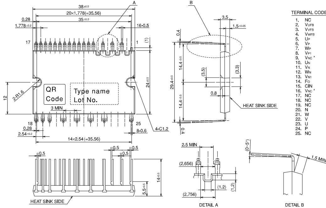
Fig. 2 LONG TERMINAL TYPE PACKAGE OUTLINES (PS21965-4A)
