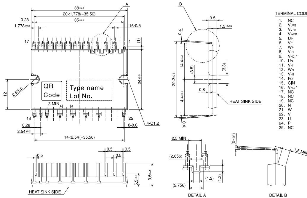
Fig. 1 PACKAGE OUTLINES (PS21965-4)
