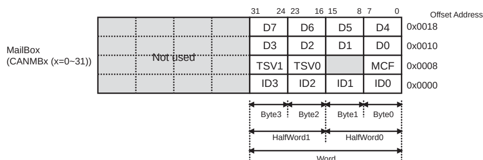
Figure 19-2 Configuration of Mailboxes
