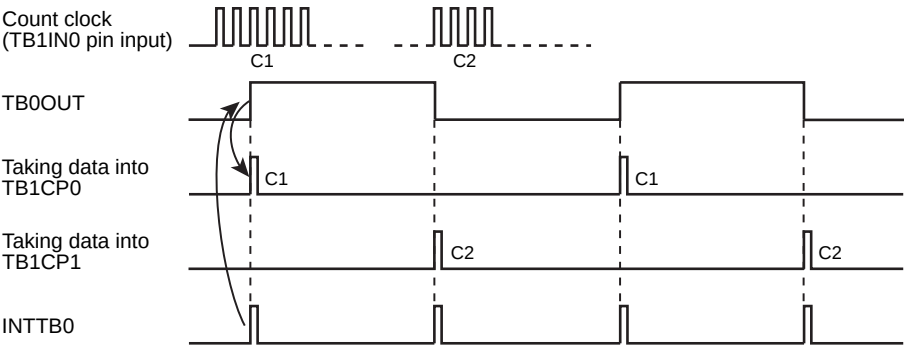
Figure 11-7 Frequency Measurement
