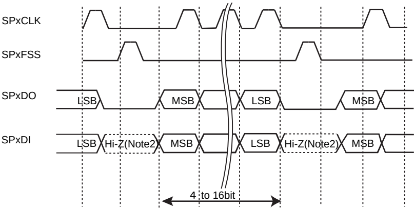
Figure 15-5 SPI frame format (continuous transfer, \langle\text{SPO}\rangle=\text{"0"} & \langle\text{SPH}\rangle=\text{"0"} )
