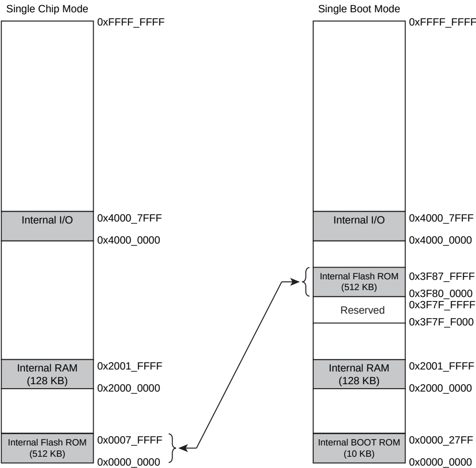
Figure 30-3 Memory Maps for TMPM368FDFG
