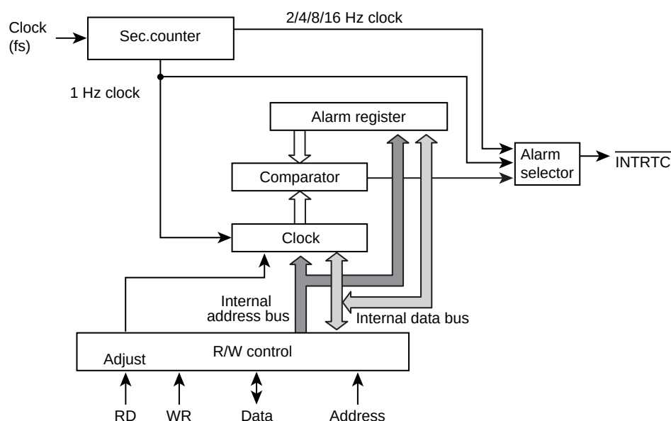
Figure 25-1 Block Diagram
