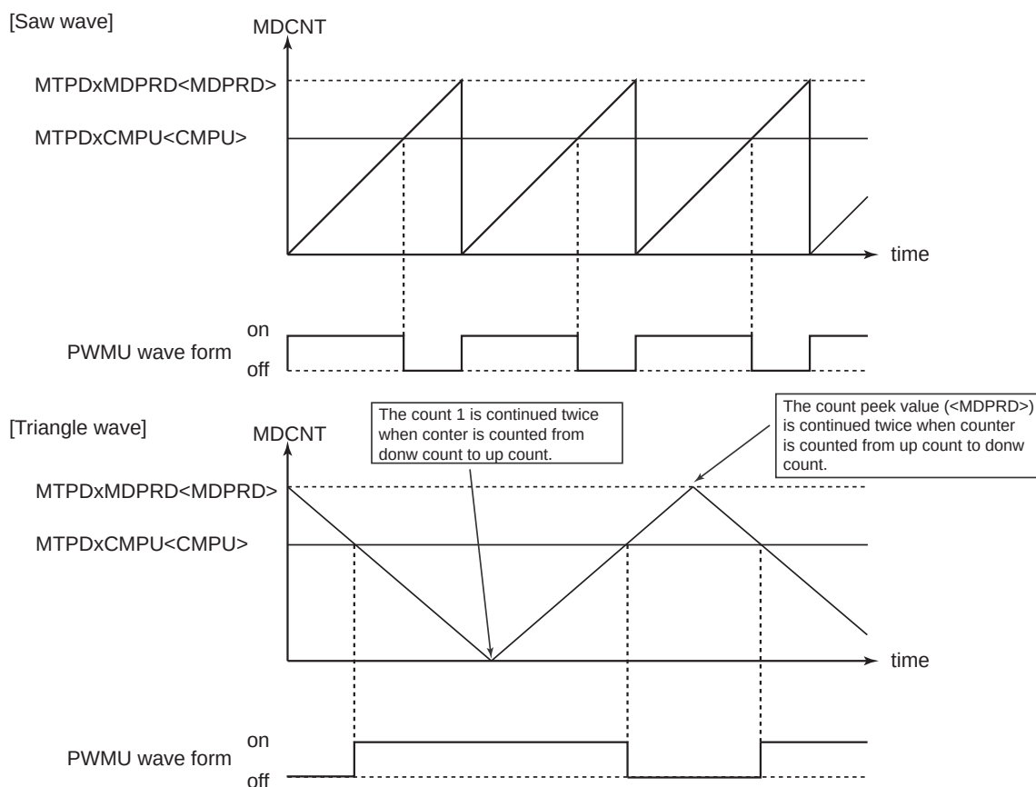
Figure 23-23 PWM waveform
