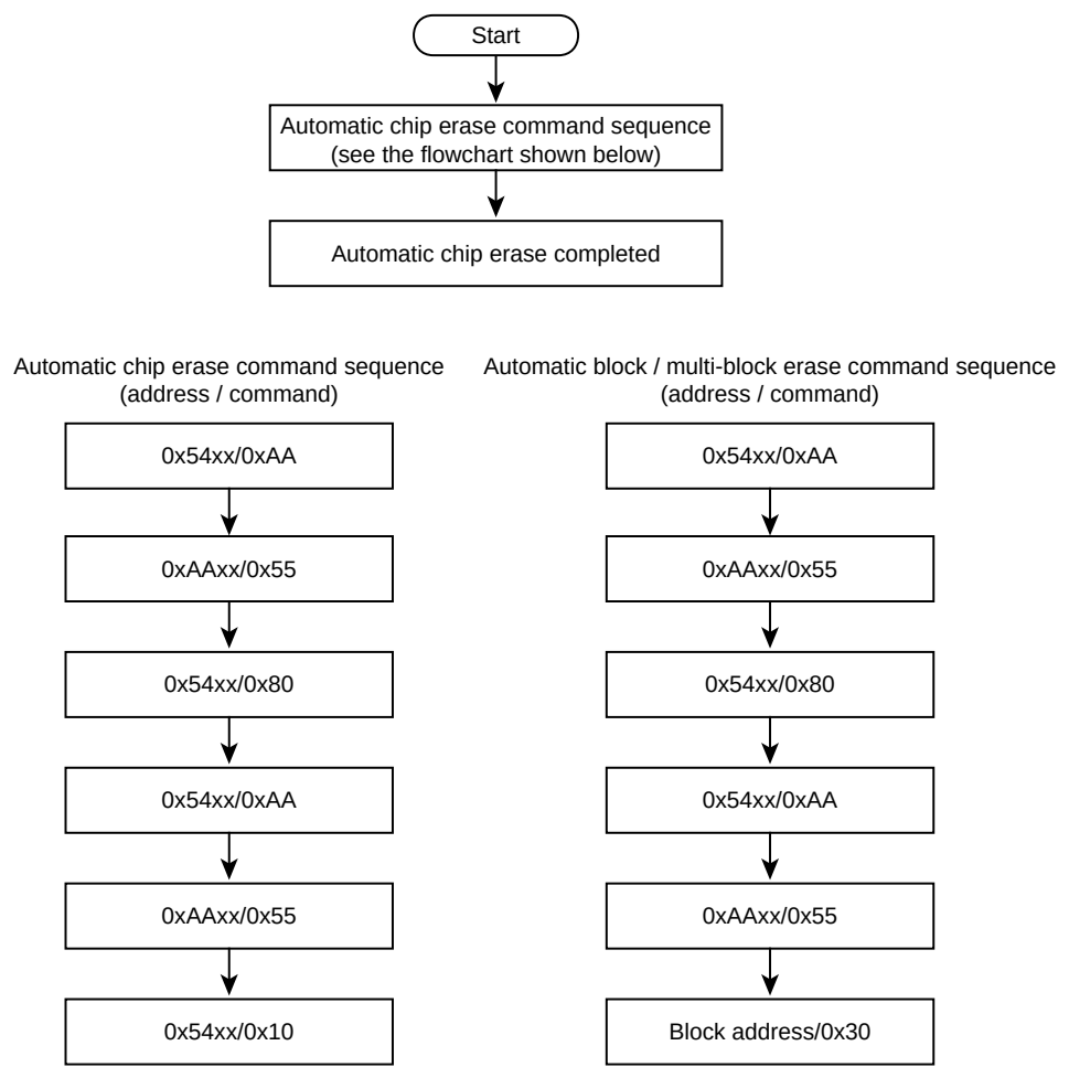
Figure 30-12 Automatic Erase
