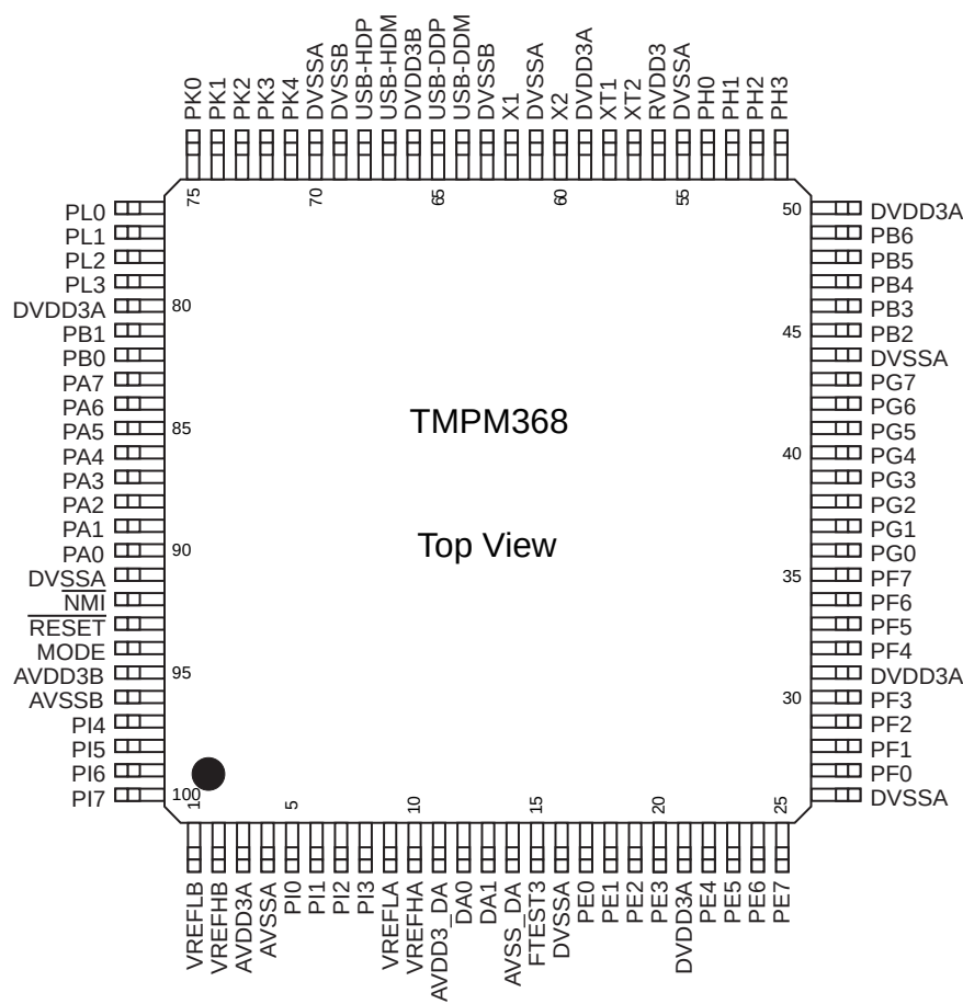
Figure 1-2 Pin Layout
