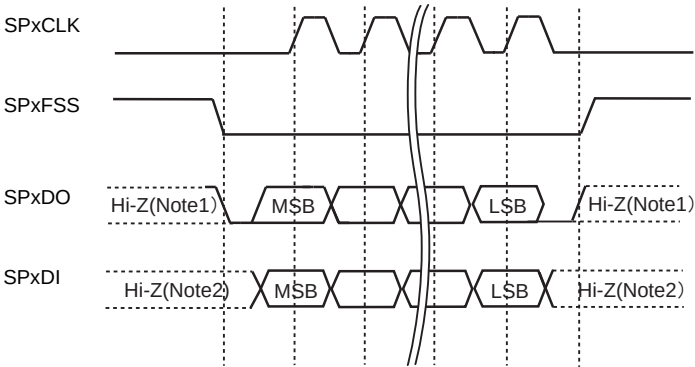
Figure 15-4 SPI frame format (single transfer, \langle\text{SPO}\rangle=\text{"0"} & \langle\text{SPH}\rangle=\text{"0"} )
