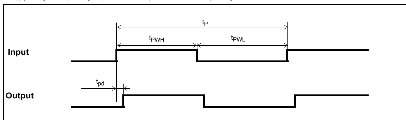
Figure 21 - Input To Output Timing
