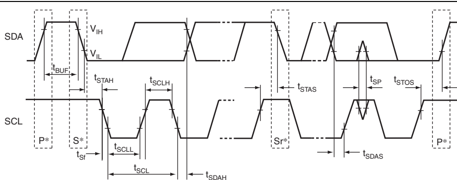
Figure 23.3 Input Timing
