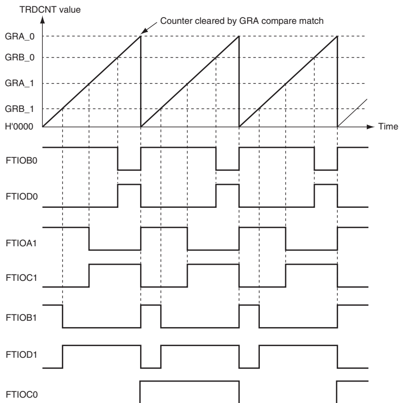
Figure 14.31 Example of Reset Synchronous PWM Mode Operation (OLS0 = OLS1 = 0)
