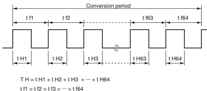
Figure 16.2 Waveform Output by 14-Bit PWM
