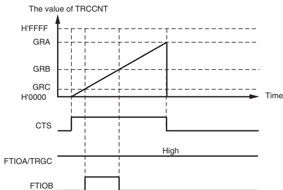
Figure 13.20 Example (1) of Output Operation of One-Shot Pulse Waveform in PWM2 Mode
