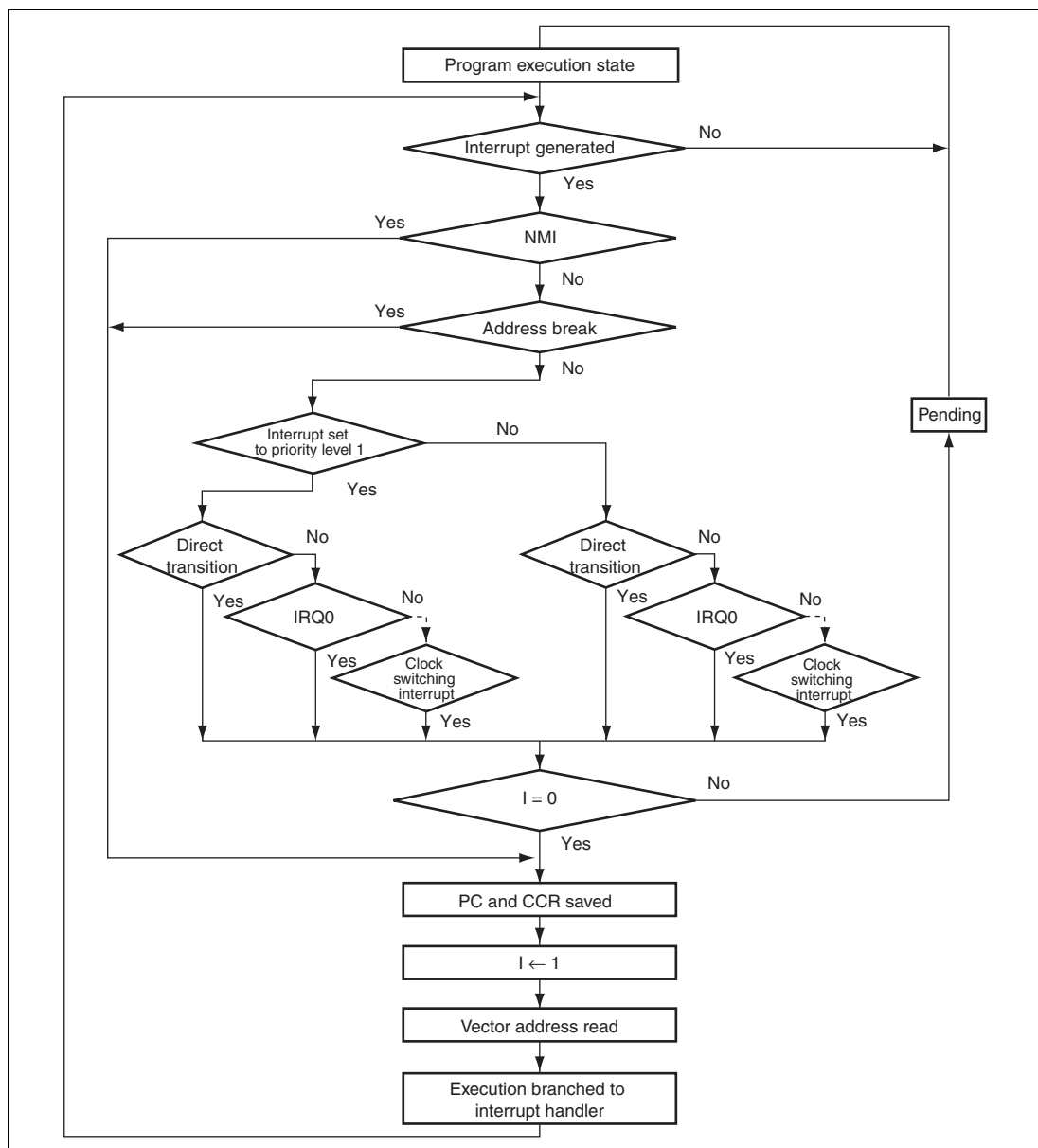
Figure 3.2 Interrupt Acceptance Flowchart
