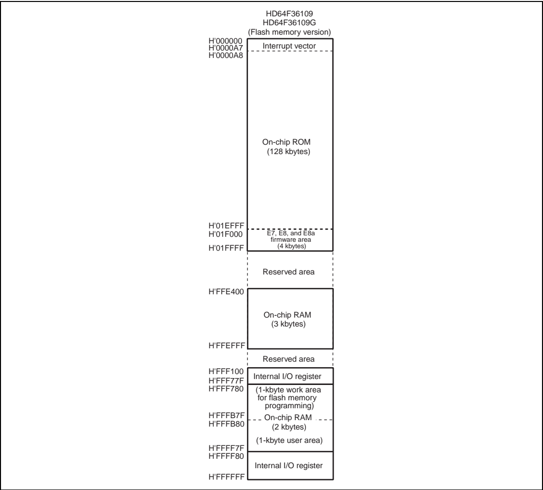
Figure 2.1 Memory Map
