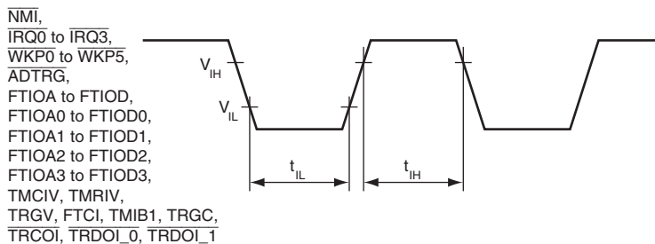
Figure 23.3 Input Timing
