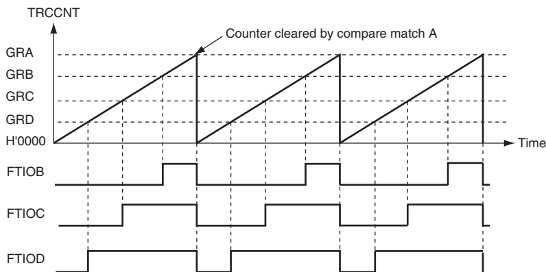
Figure 13.10 PWM Mode Example (2)
