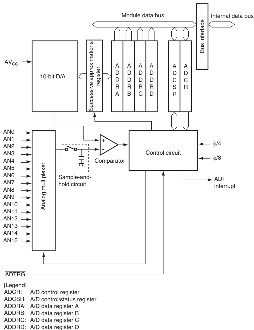
Figure 19.1 Block Diagram of A/D Converter
