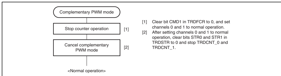
Figure 14.33 Canceling Procedure of Complementary PWM Mode
