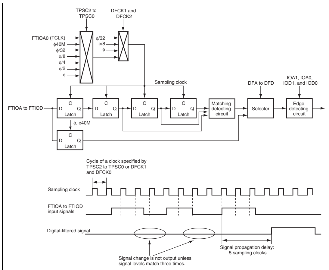
Figure 14.54 Block Diagram of Digital Filter
