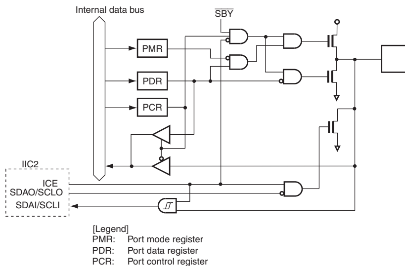
Figure B.12 Port5 Block Diagram (P57, P56)
