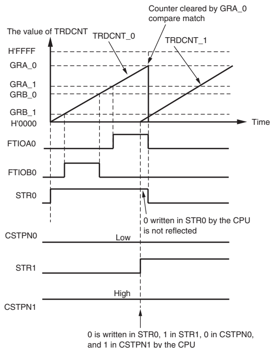
Figure 14.6 Example of Starting and Stopping Operations of Counters (in PWM3 Mode)
