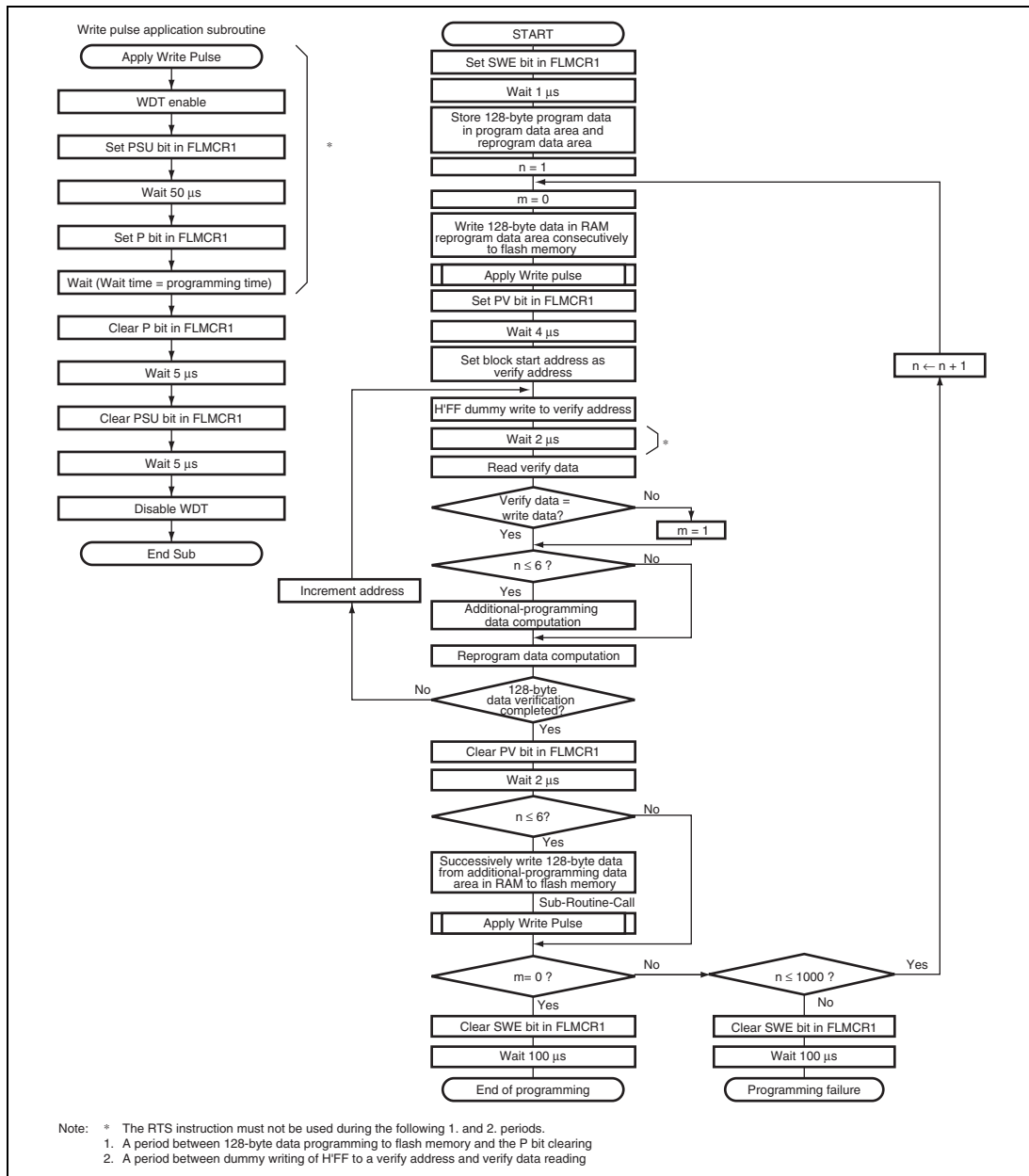
Figure 7.3 Programming/Program-Verify Flowchart
