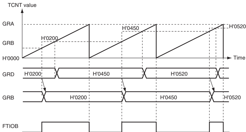
Figure 13.11 Buffer Operation Example (Output Compare)
