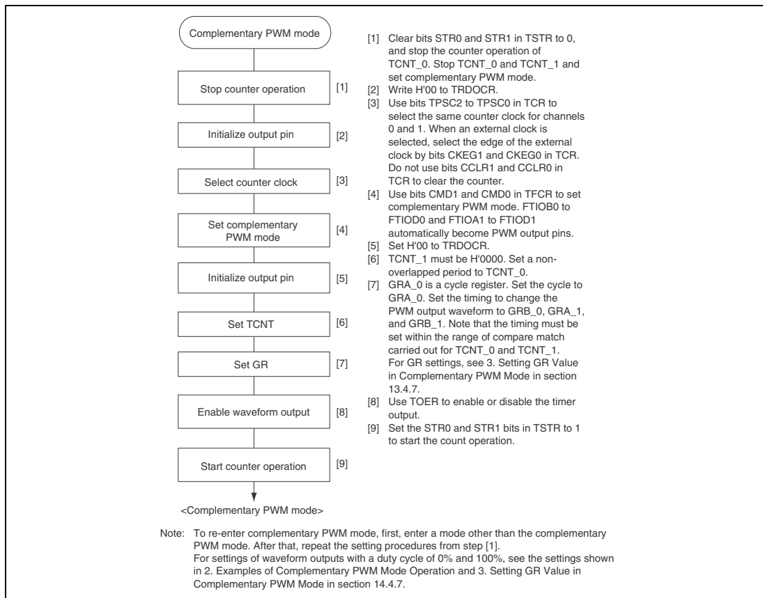
Figure 14.32 Example of Complementary PWM Mode Setting Procedure
