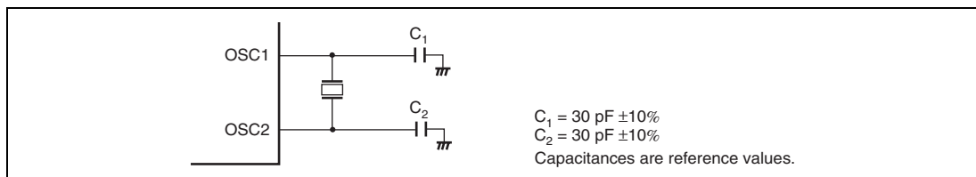
Figure 5.12 Example of Connection to Ceramic Resonator
