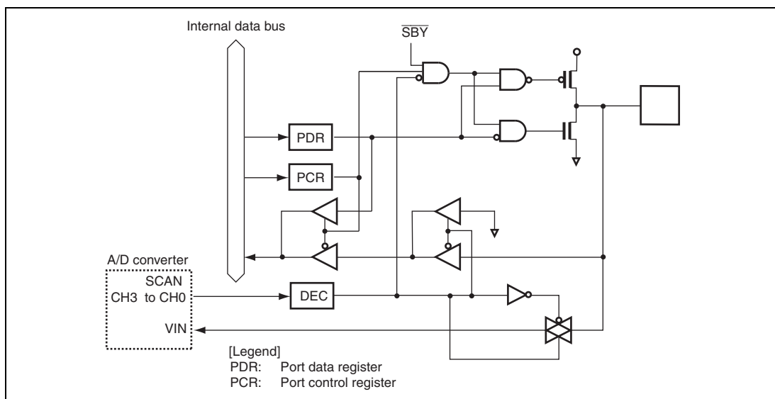
Figure B.27 Port G Block Diagram (PG4, PG3, PG2, PG1, PG0)
