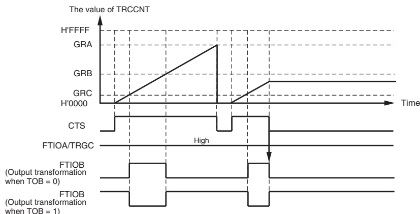
Figure 13.19 Example of Stopping Operation of the Counter in PWM2 Mode
