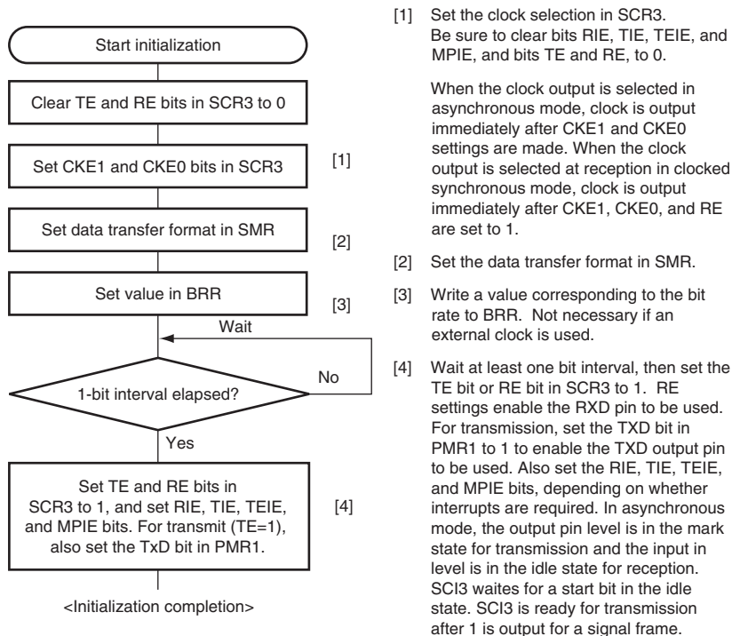
Figure 17.4 Sample SCI3 Initialization Flowchart
