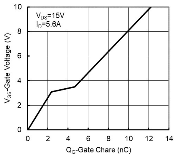
Figure6. Gate Charge
