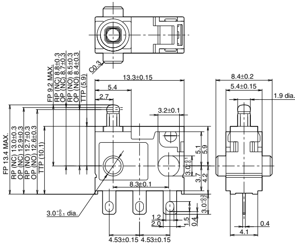
External dimensions
