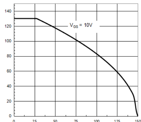
Figure 4. Drain Current
