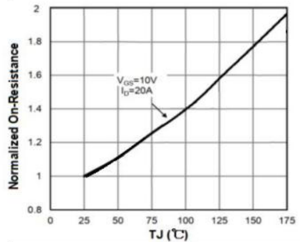
Figure 4 Rdson-JunctionTemperature
