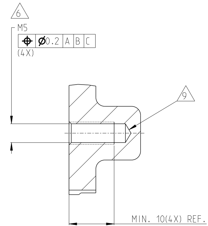
SECTION B-B
