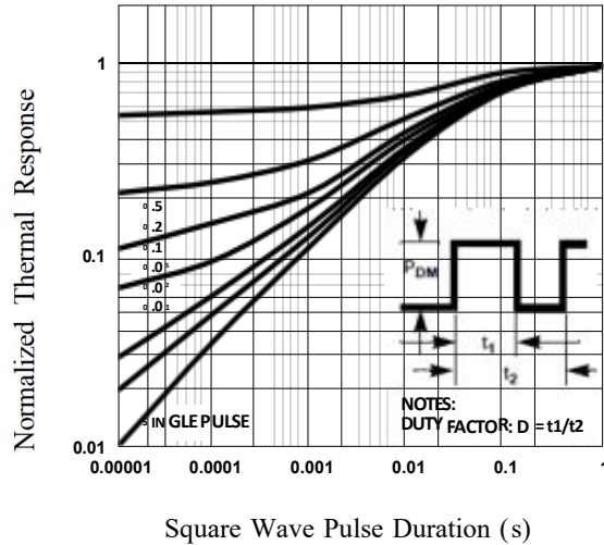
Fig. 9 Normalized Transient
