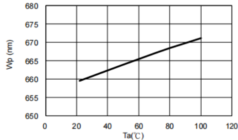
Fig.5-Peak Wavelength (@20mA) vs. Ambient Temperature
