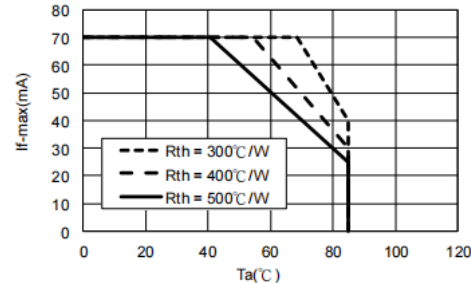
Fig.6- Maximum Driving Forward DC Current vs. Ambient Temperature(Derating based on T_J \text{ max}=110^{\circ}\text{C} )
