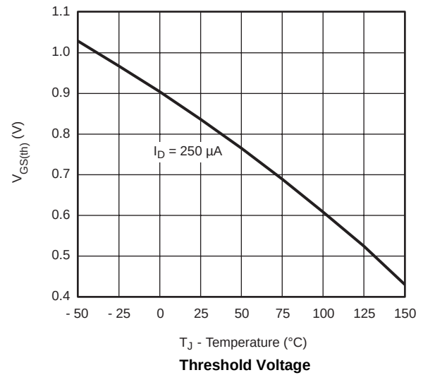
Threshold Voltage
