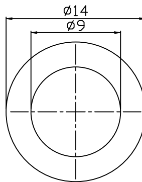
WASHER 1pcs
