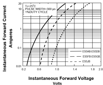
FIG. 3-TYPICAL FORWARD VOLTAGE CHARACTERISTICS
