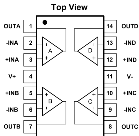
Fig.5-5. GT324: TD(TSSOP14) Package
