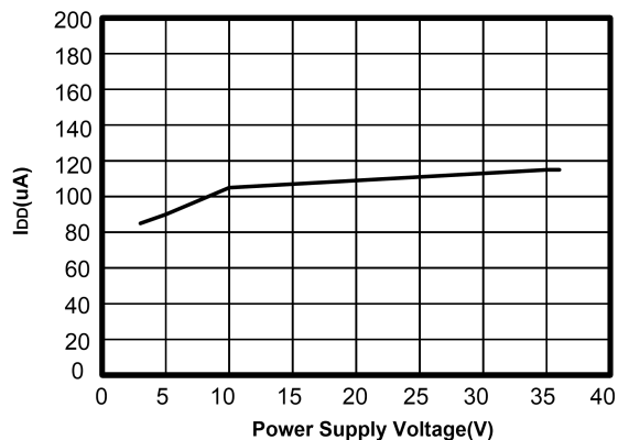
Fig.8-6. I_Q vs Power Supply Voltage(25°C)
