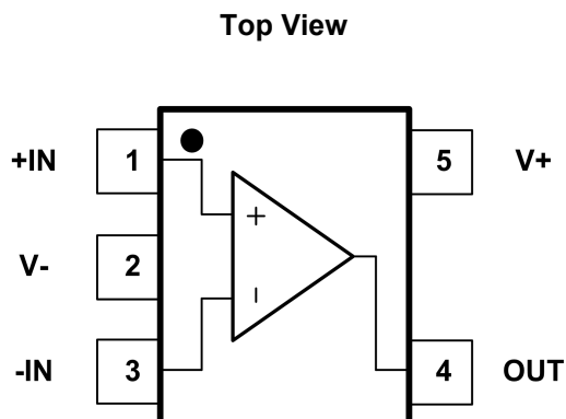
Fig.5-1. GT321: S5(SOT23-5) Package
