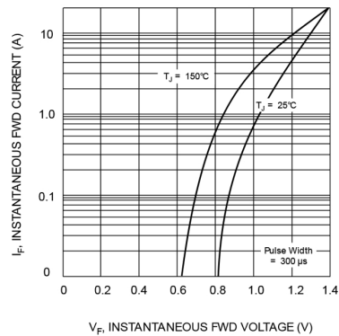
Fig. 2 Typical Fwd Characteristics
