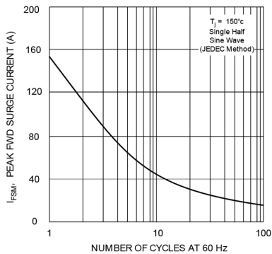
Fig. 3 Max Non-Repetitive Peak Fwd Surge Current
