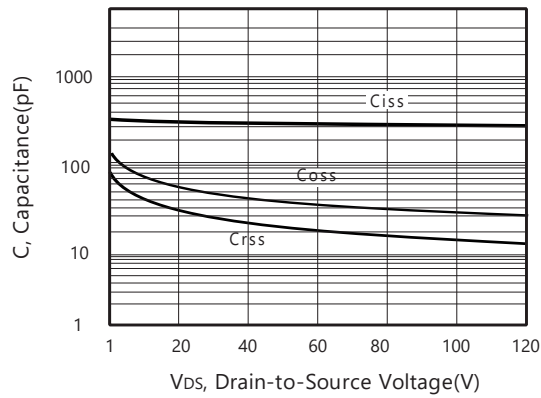
Figure 7. Capacitance
