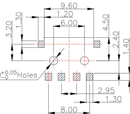
P.C.B.MOUNTING DETAIL
