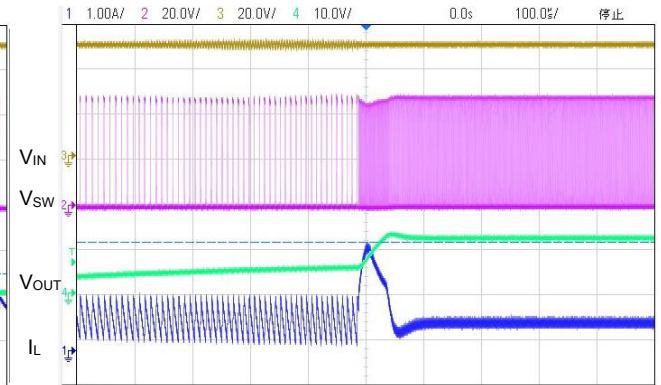
(22) Short Output Recovery (VIN=50.0V, OUT=12V, IOUT=0.6A)
