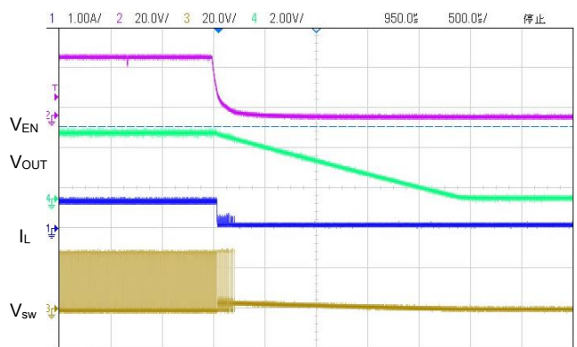
(18) Enable Shutdown(VIN=30.0V,VOUT=3.3V,IOUT=0.6A)
