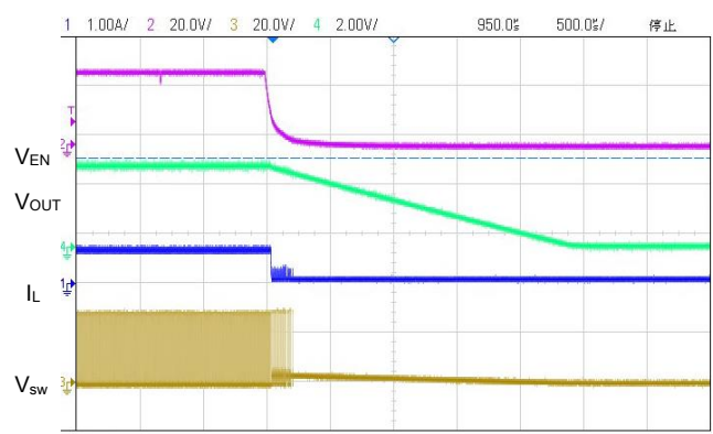
(18) Enable Shutdown(VIN=30.0V,VOUT=3.3V,IOUT=0.6A)
