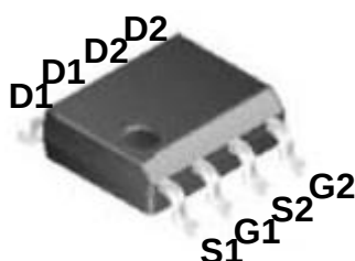
SOP8 Pin Configuration
