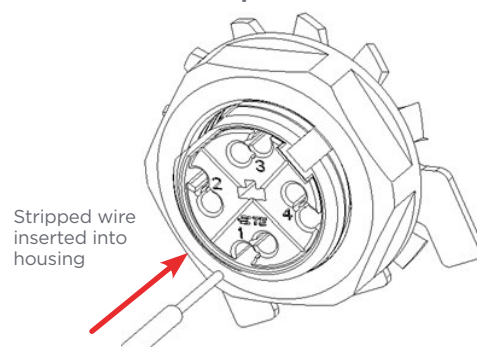
Wire poke-in locations (4)
