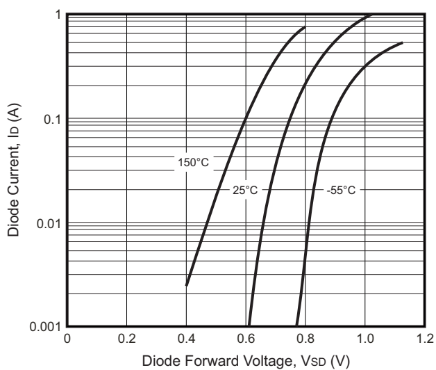
Fig.3 - Body Diode Current vs. Body Diode Voltage
