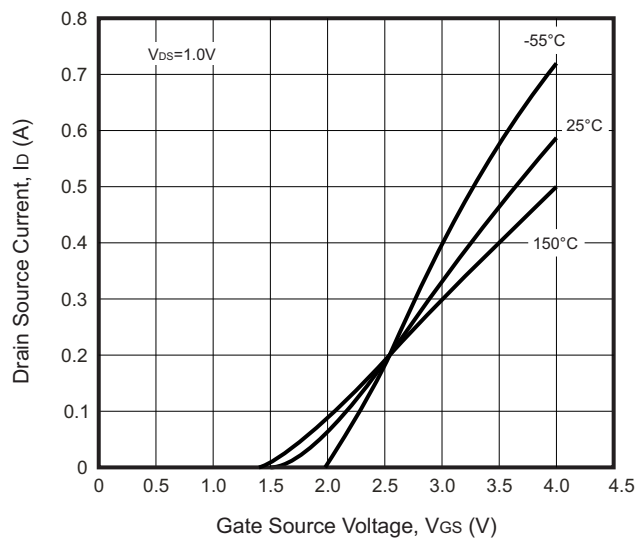
Fig.2 - Transfer Characteristics
