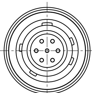
A10YDR-P07XCDO-0000 Mechanical coding: D Color coding: green
