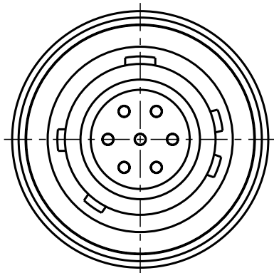
A10YBR-P07XCDO-0000 Mechanical coding: B Color coding: red
