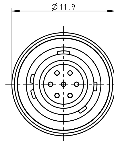
A10YAR-P07XCDO-0000 Mechanical coding: A Color coding: light brown
