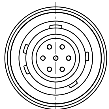
A10YCR-P07XCDO-0000 Mechanical coding: C Color coding: blue
