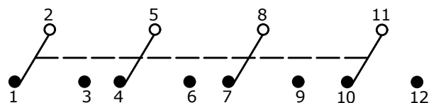
CIRCUIT: 4PDT
