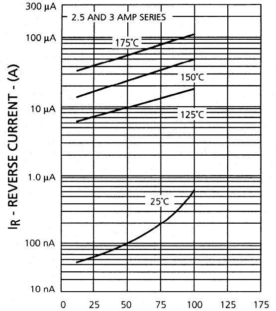
Percent V_R Rating FIGURE 4 Typical Reverse Current vs. Applied Reverse Voltage
