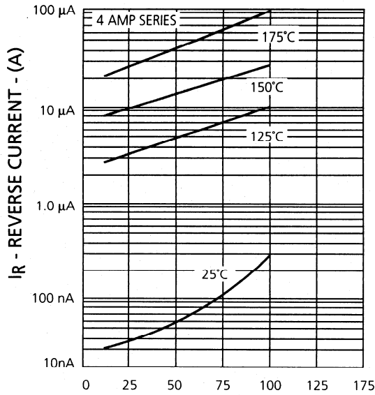
Percent V_R Rating FIGURE 3 Typical Reverse Current vs. Applied Reverse Voltage
