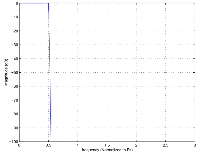
Figure 9-13. Stopband—ASRC, Notch Disabled
