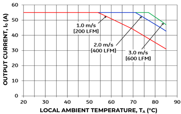
Figure 21. Output Current Derating for the Base plate QBDE055A0Bxx-H+0.5" Heat Sink in the Transverse Orientation; Airflow Direction for input- to input+ orientation; V_{in} = 50V . Current
