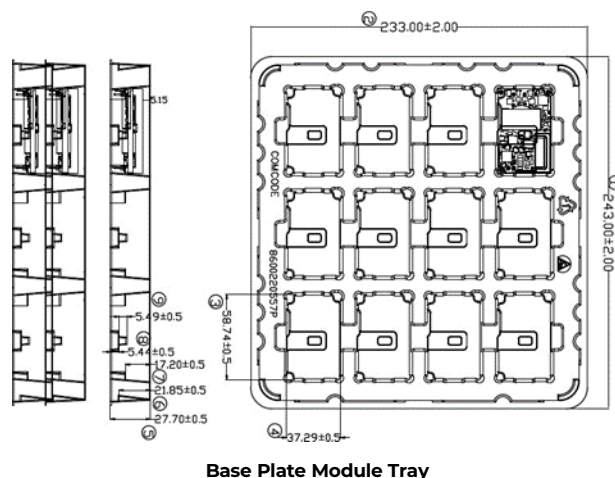
Figure 27. QBDE055A0B Packaging Tray
