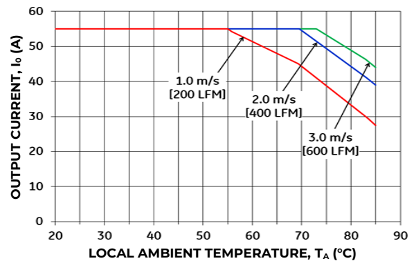
Figure 22. Output Current Derating for the Base plate QBDE055A0B_DSxx-H+0.5" Heat Sink in the Longitudinal Airflow Direction for input to output orientation; V_{in} = 50V .
