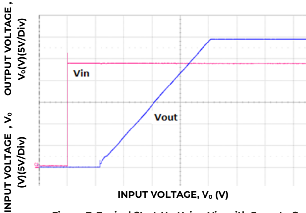
Figure 7. Typical Start-Up Using V_{in} with Remote On/Off enabled, negative logic version, with the -P option shown, I_o = 33.5 I_{o,max} .
