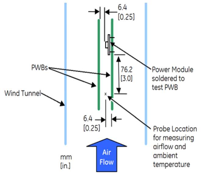
Figure 18. Thermal Test Setup.
