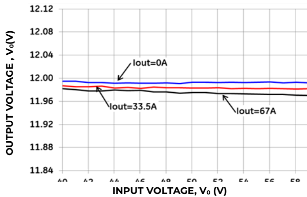
Figure 9. Typical Output Voltage Regulation vs. Input Voltage without the -P option.
