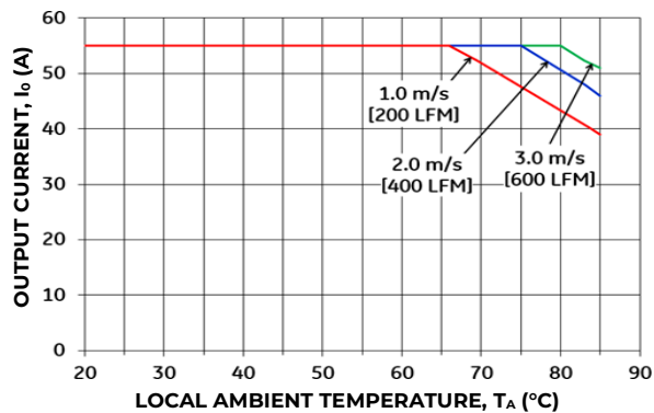
Figure 23. Output Current Derating for the Base plate QBDE055A0Bxx-H+1.0" Heat Sink in the Transverse Orientation; Airflow Direction for input- to input+; V_{in} = 50V .
