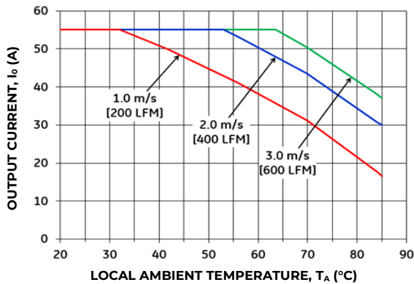
Figure 19. Output Current Derating for the Base plate QBDE055A0B_DSxx-H in the Transverse Orientation; Airflow Direction for input- to input+ orientation; V_{in} = 50V
