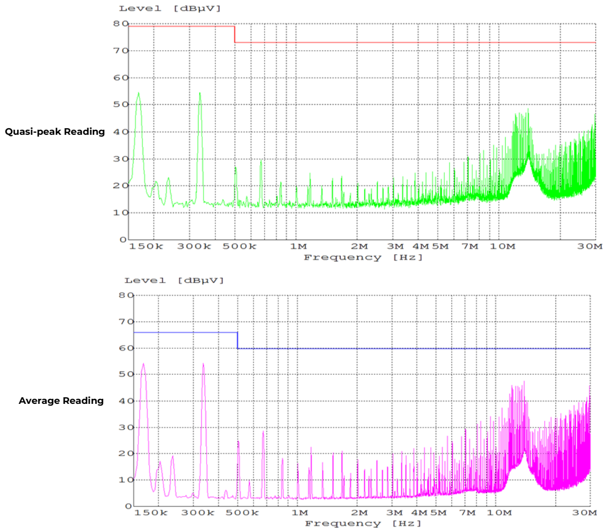
Figure 26 : EMC Consideration
