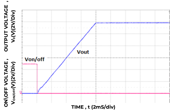
Figure 8. Typical Start-Up Using Remote On/Off with V_{in} applied, negative logic version, with the -P option shown, I_o = 33.5 I_{o,max} .
