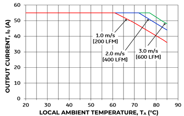
Figure 24. Output Current Derating for the Base plate QBDE055A0Bxx-H+1.0" Heat Sink in the Longitudinal Airflow Direction for input to output orientation; V_{in} = 50V .
