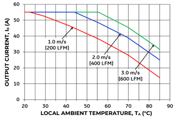
Figure 20. Output Current Derating for the Base plate QBDE055A0B_DSxx-H in the Longitudinal Airflow Direction for input to output orientation; V_{in} = 50V .
